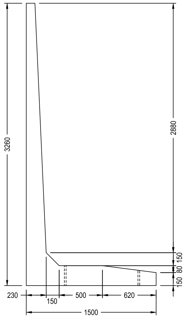
End View
